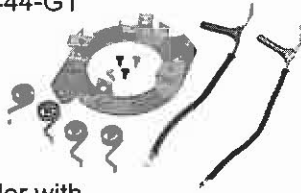
Brush holder with springs and crossover studs
